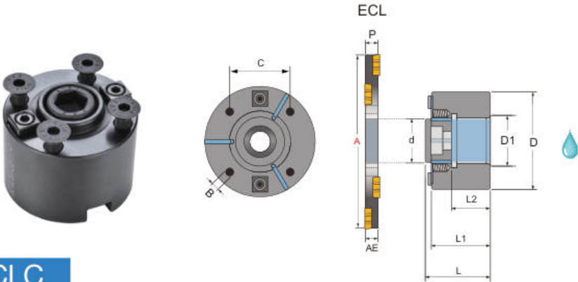
Coolant Inlet and Outlet Direction
