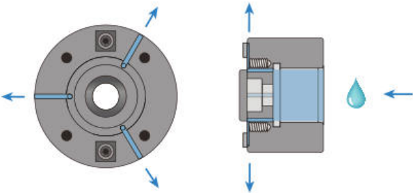
Coolant Inlet and Outlet Direction
