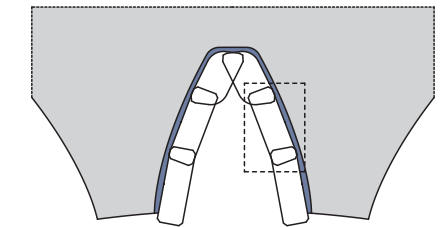
IV Schrappen angepasste Kontur Roughing of internal gears with adapted contour
