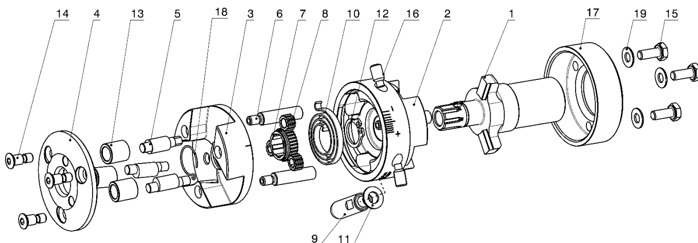
Figure 22: Exploded view F01
