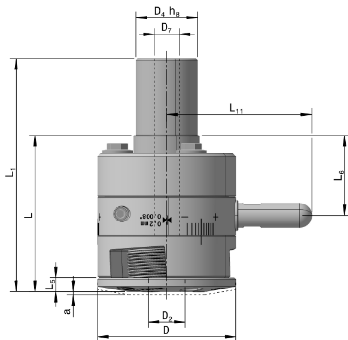
Figure 10: Dimensions of the rolling system
