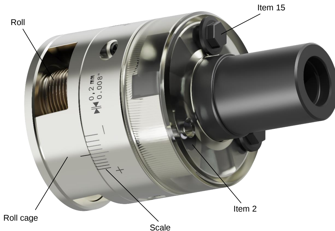
Figure 12: Adjustment scale on the housing of the axial rolling system
